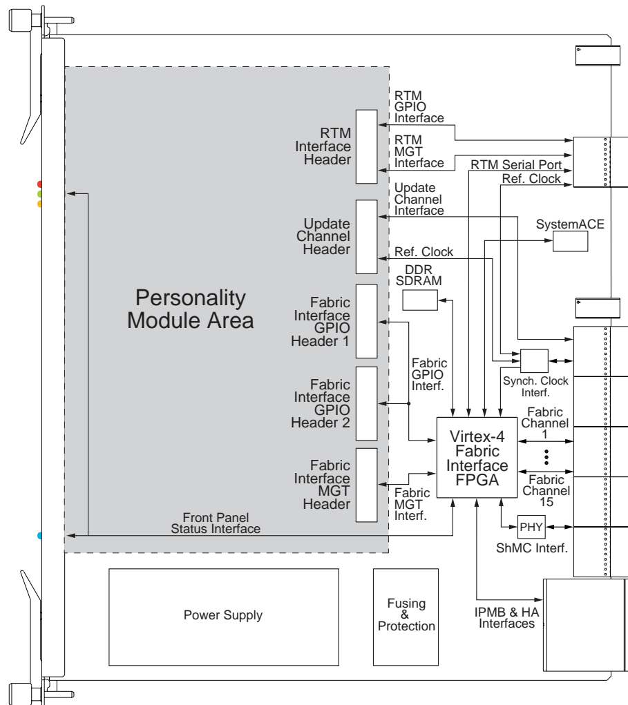
Figure 1 Full-Mesh Line Card Block Diagram
